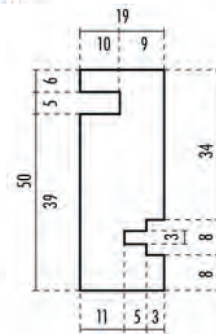
C profilo architrave
